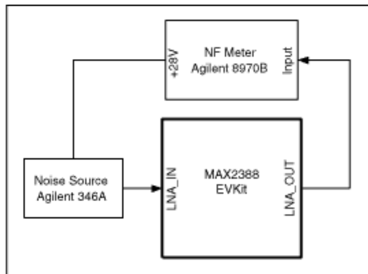
Figure 3. MAX2388 LNA NF measurement.
