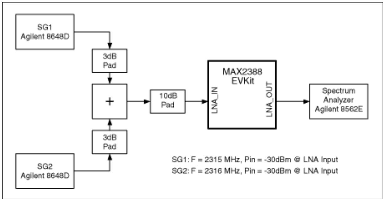
Figure 1. MAX2388 LNA IIP3 measurement.
