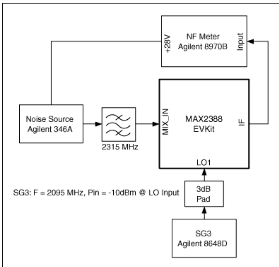
Figure 4. MAX2388 mixer NF measurement.
