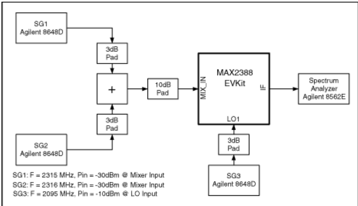
Figure 2. MAX2388 mixer IIP3 measurement.
